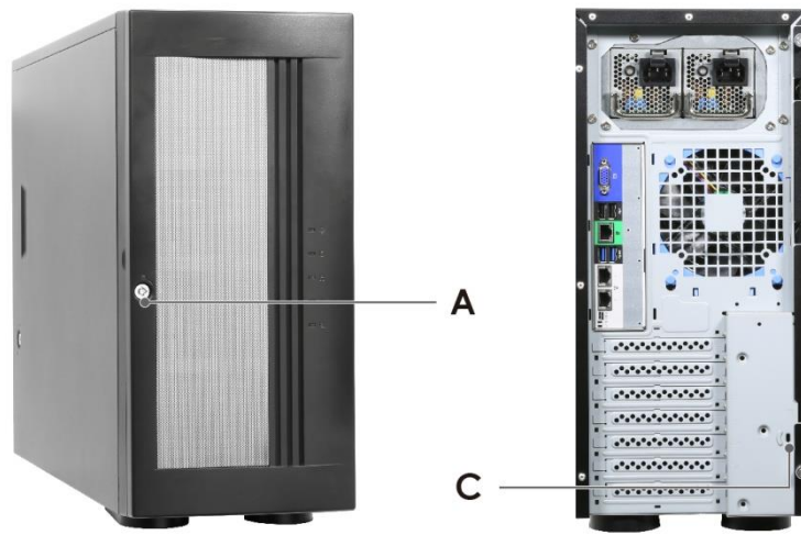
Figure 5 Key lock and Kensington slot location
