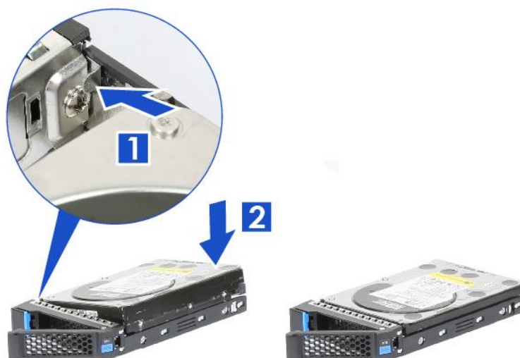
Figure 23 3.5" HDD installation (tool-less type)
