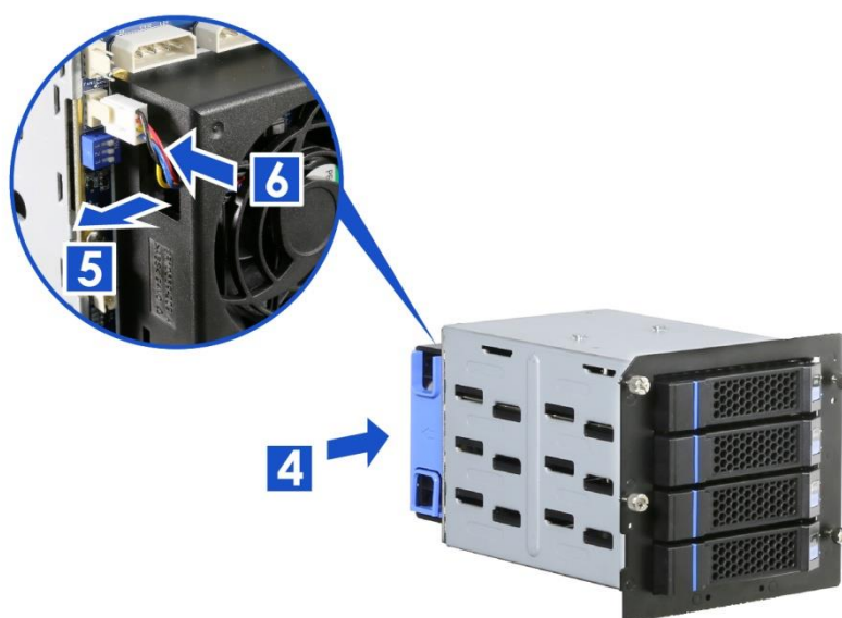
Figure 20 3.5" hot-swap HDD cage fan maintenance step-2
