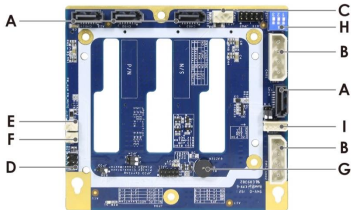
Figure 36 Backplane rear view
