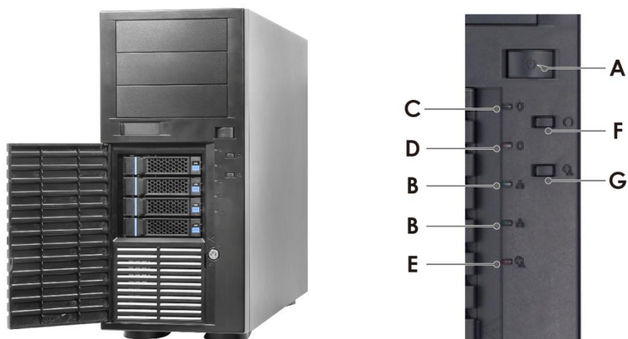
Figure 8 Front control panel
