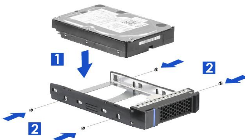
Figure 24 3.5" HDD installation (screw type)
