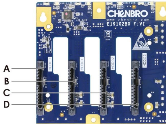
Figure 35 Backplane front view
