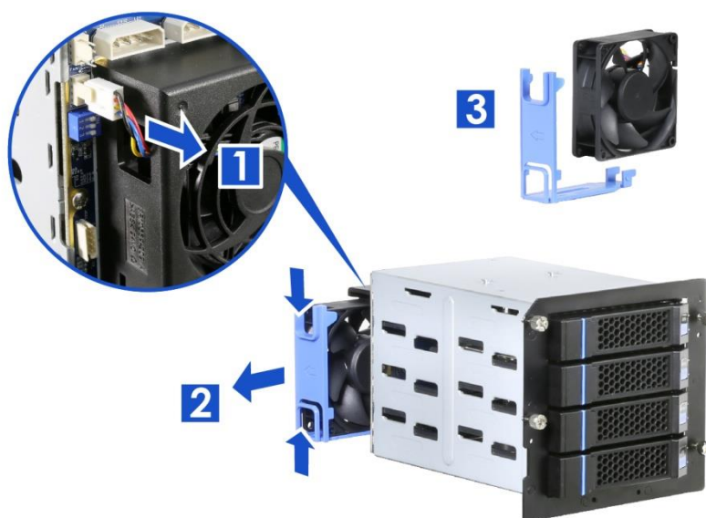
Figure 19 3.5" hot-swap HDD cage fan maintenance step-1
