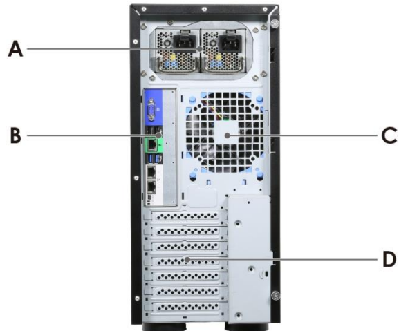
Figure 3 Back panel with redundant PSU
