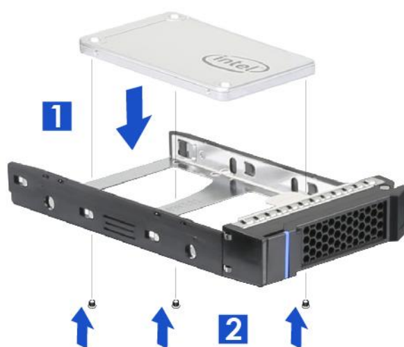
Figure 25 2.5" HDD/SSD installation (screw type)
