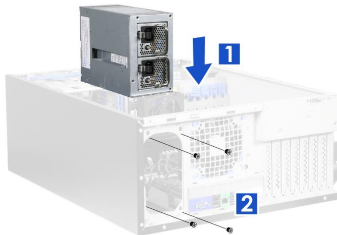
Figure 31 Redundant PSU installation
