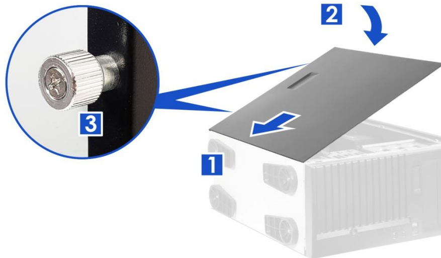
Figure 11 Side cover installation
