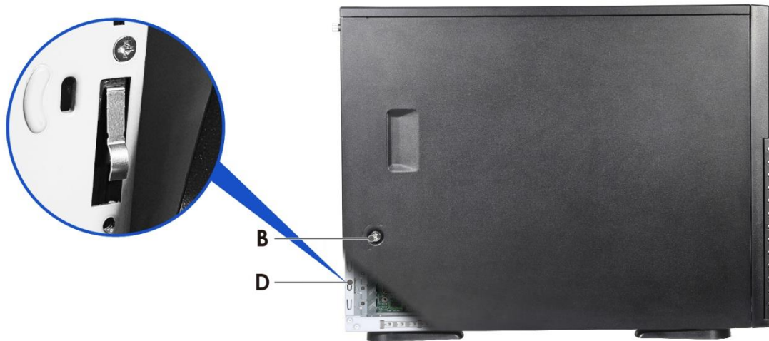
Figure 6 Intrusion switch location
