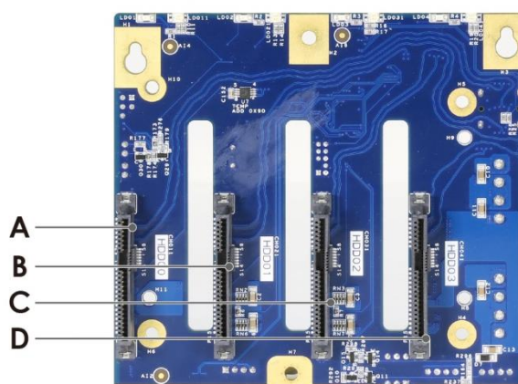
Figure 33 Backplane front view
