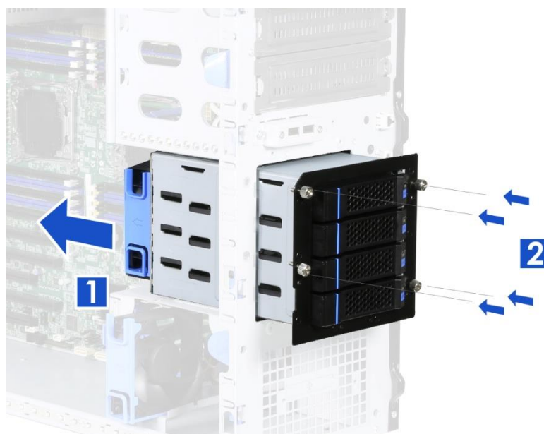
Figure 18 3.5" hot-swap HDD cage installation
